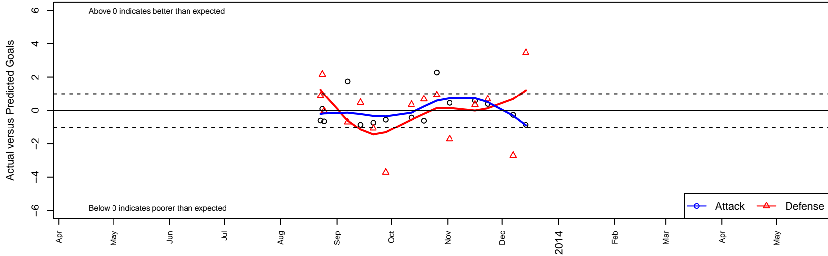
BIFC White B02 Dots are actual minus expected GF (blue circles) and GA (red triangles). Blue line is smoothed change in attack strength. Red is smoothed change in defense strength.
